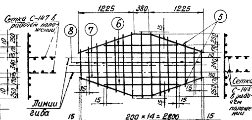
C-149
